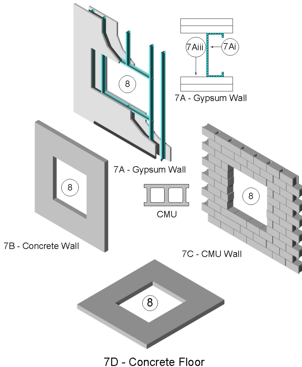
Figure 5 – Supporting Constructions
