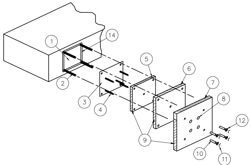
Field Fabricated Door System
